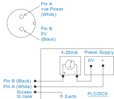
Connection Details
