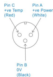
Connection Details
